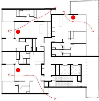
L 3-4 SCALE 1:200
